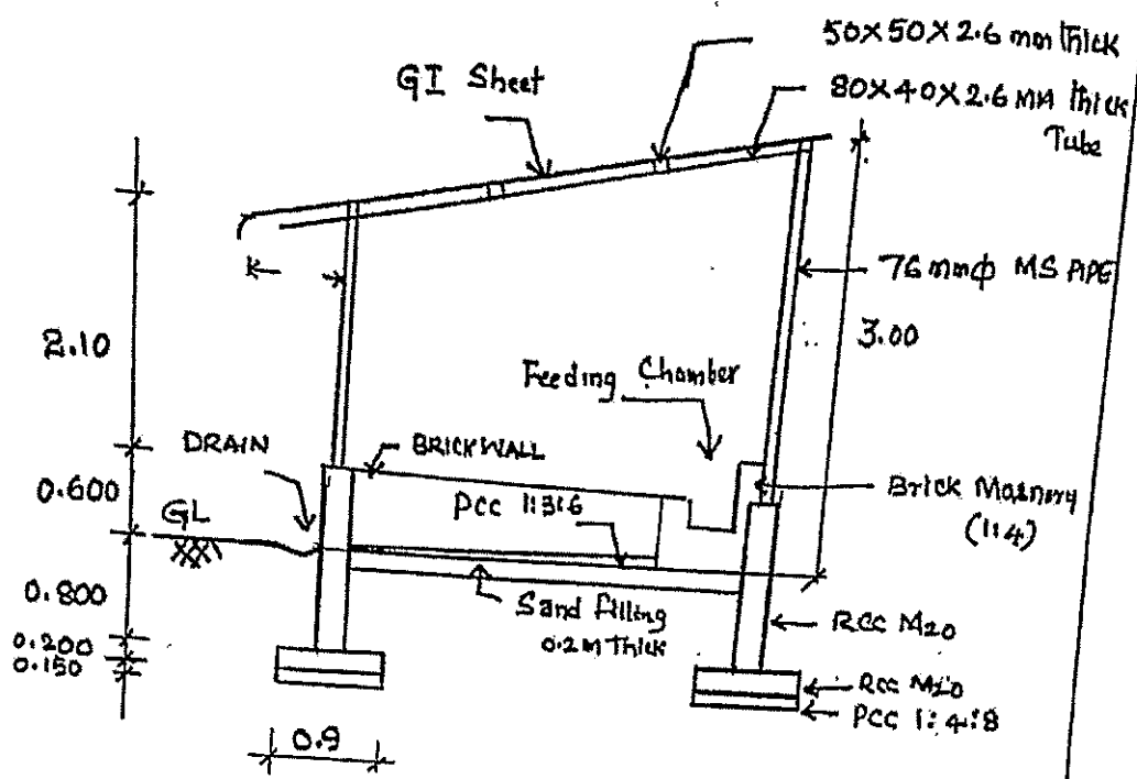
CROSS SECTION
